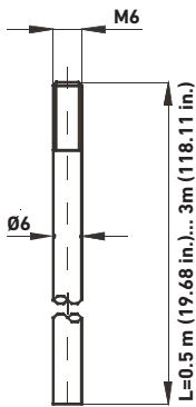
Probe dimension
