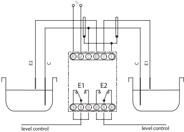
Device Settings
