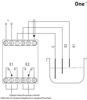
Level Control - Two levels in one tank
